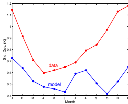
Fig. 24: Monthly standard deviations of the Niño-3.4 SST index calculated from the 100-yr synchronous CCSM2/T31x3a integration phase (blue) and from 1950–2004 NCEP data (red).
