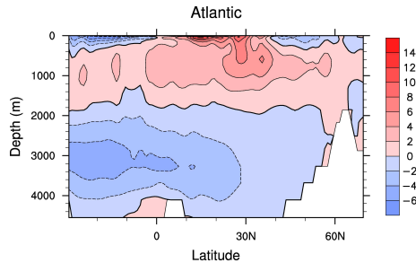
Fig. 1: Atlantic meridional overturning circulation ( Sv ) obtained with the Eulerian-mean velocity from the standard CCSM2.0.1 low-resolution control run with default settings and parameters. A 10-yr average is shown calculated from years 278–287 (the control run has started from observational data).
