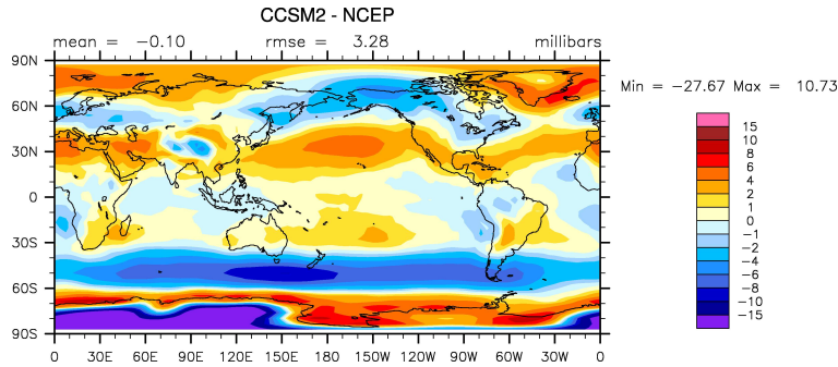
Fig. 16: Difference in annual-mean sea-level pressure between CCSM2/T31x3a and NCEP 1979–1998 reanalysis data (rmse = root-mean-square error).
