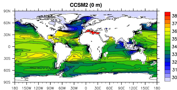
Fig. 2: Annual-mean sea surface salinity ( psu ) in the standard CCSM2.0.1 low-resolution control run with default settings and parameters. A 10-yr average is shown calculated from years 278–287 of the simulation. The model output can be compared with observations shown in Figure 12.
