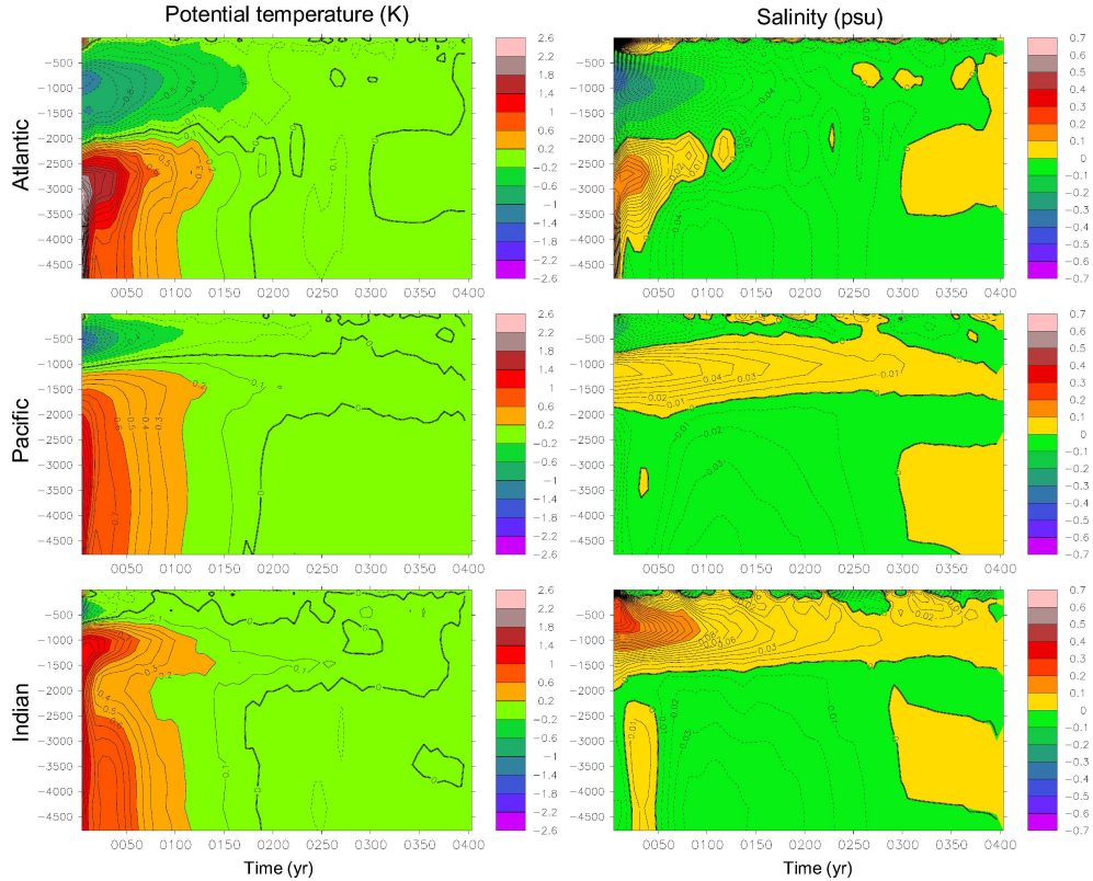
Fig. 6: Time versus depth ( m ) plots of horizontally averaged potential temperatures (left) and salinities (right) for the Atlantic, Pacific, and Indian Ocean basins, plotted as deviations from the mean value of year 400 (smoothed by 7-yr averaging). Contour intervals are 0.1 K and 0.01 psu, respectively. Note that deep-ocean acceleration is applied from (surface) year 8 to (surface) year 300.
