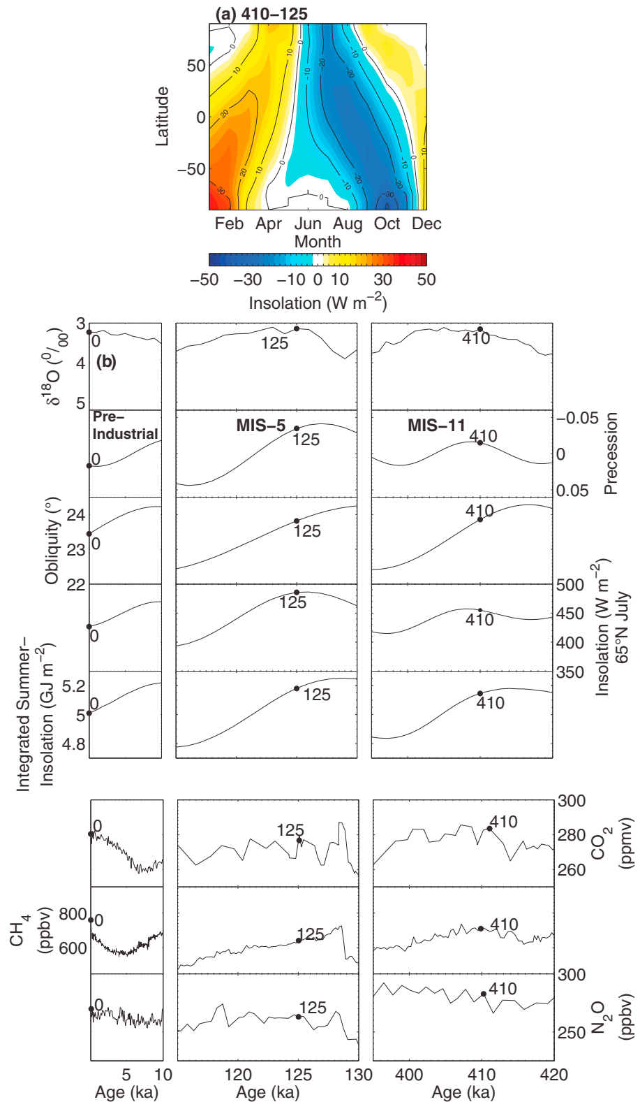
Figure 1. (a) Insolation anomalies between 410 and 125 ka. The calculation assumes a fixed present-day calendar with vernal equinox at 21 March. (b) Benthic \delta^{18}O stack (Lisiecki & Raymo, 2005), climatic precession, obliquity, July insolation at 65°N (Berger, 1978), the integrated summer insolation with \tau=275 W/m^2 according to Huybers (2006), and GHG concentrations (Louergue et al., 2008; Lüthi et al., 2008; Schilt et al., 2010) for the Holocene, MIS 5e, and MIS 11. GHG concentrations for the industrial era are not shown. The dots mark the time slices simulated in this study.
